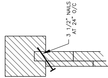
FENCE POST DETAIL SECTION 'A'-'A'
