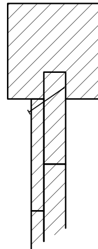
FENCE POST DETAIL SECTION 'A'-'A'
