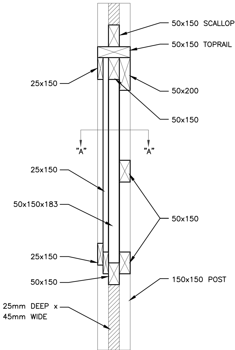
CROSS-SECTION OF WOOD ACOUSTIC FENCE
