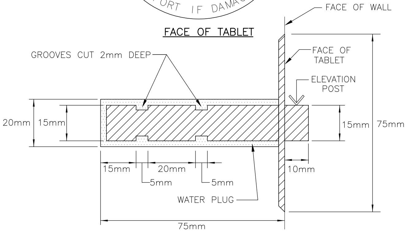
CROSS SECTION
